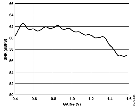
Figure 11. SNR vs. GAIN+, AOUT = -1.0 dBFS
