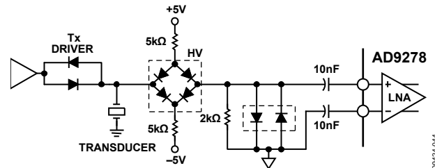
Figure 47. Input Overload Protection
