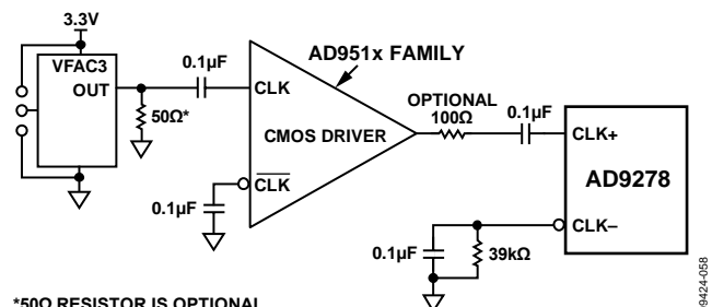
Figure 53. Single-Ended 1.8 V CMOS Sample Clock
