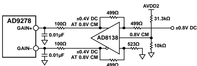
Figure 49. Differential GAIN_{\pm} Pin Configuration
