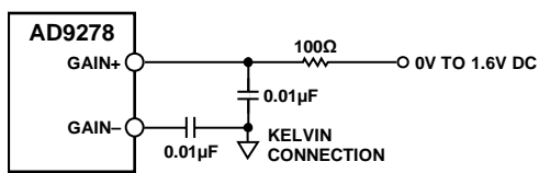
Figure 48. Single-Ended GAIN_{\pm} Pin Configuration
