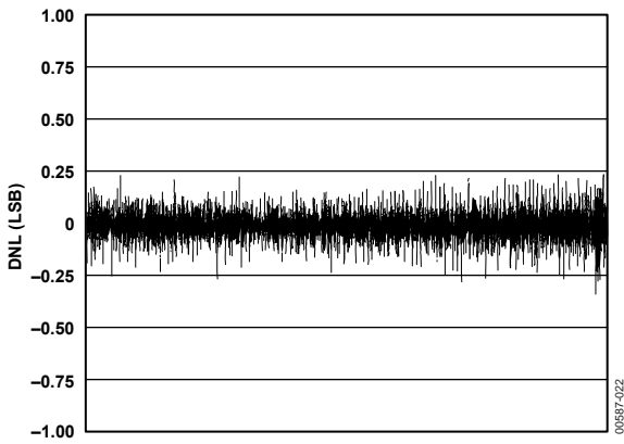
Figure 18. Differential Nonlinearity, f_s = 105 MSPS
