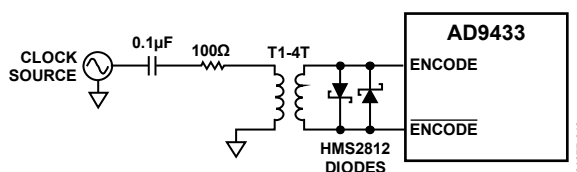
Figure 43. Transformer-Coupled Encode Circuit
