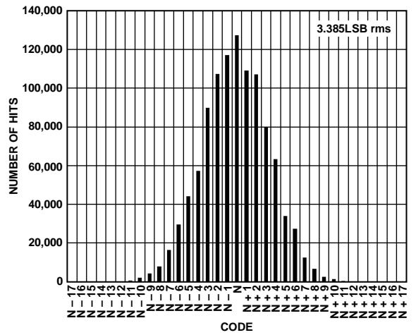
Figure 21. Input-Referred Noise Histogram, 2.5 \text{ V p-p FS}
