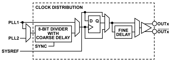
Figure 32. Clock Distribution Paths for PLL1, PLL2, and SYSREF Frequency Sources
