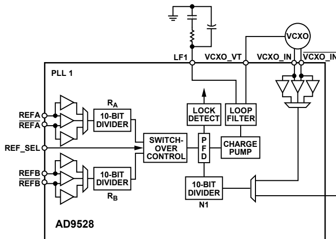
Figure 29. Input PLL (PLL1) Block Diagram
