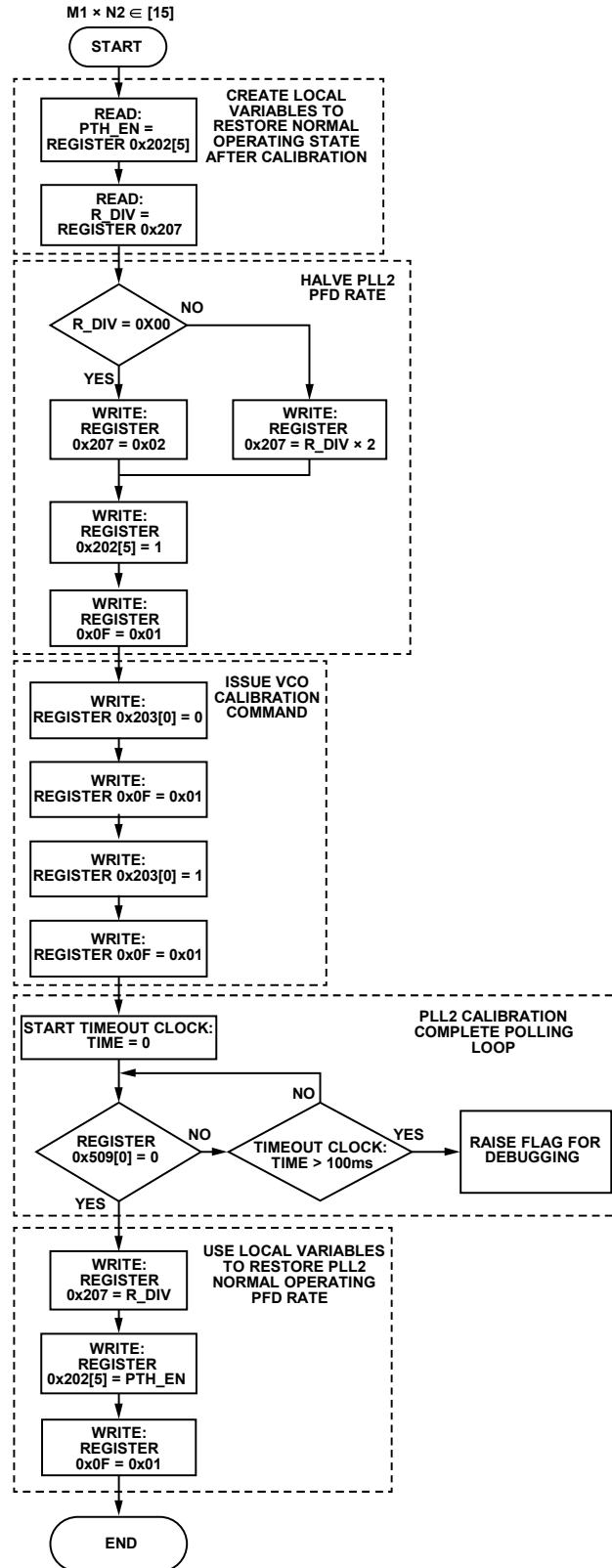
Figure 54. Subprocess, Issue VCO Calibration (M1 × N2 = 15)
