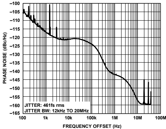
Figure 3. Absolute Phase Noise, f_R = 10\text{ MHz} , f_{OUT} = 122.88\text{ MHz} , 3.3\text{ V CMOS} Single-Ended Input, HSTL Output, Fractional-N PLL Mode, Internal VCO, LBW = 100\text{ kHz}
