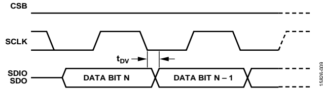
Figure 56. Timing Diagram for Serial Control Port Register Read—MSB First
