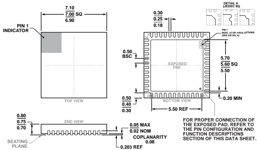
COMPLIANT TO JEDEC STANDARDS MO-220-WKKD-4. Figure 65. 48-Lead Lead Frame Chip Scale Package [LFCSP] 7 mm x 7 mm Body and 0.75 mm Package Height (CP-48-13) Dimensions shown in millimeters
