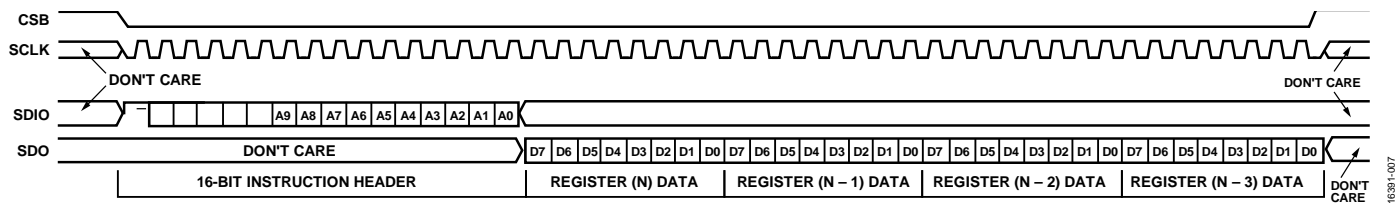
Figure 54. Serial Control Port Read—MSB First, Address Decrement, Four Bytes of Data
