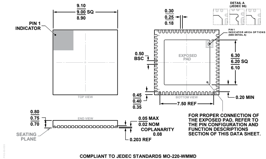
COMPLIANT TO JEDEC STANDARDS MO-220-WMMD Figure 44. 64-Lead Lead Frame Chip Scale Package [LFCSP] 9 mm × 9 mm and 0.75 mm Package Height (CP-64-17) Dimensions shown in millimeters
