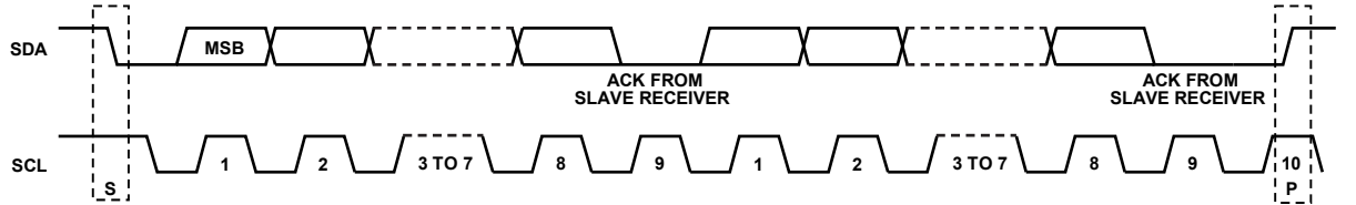
Figure 35. Acknowledge Bit
