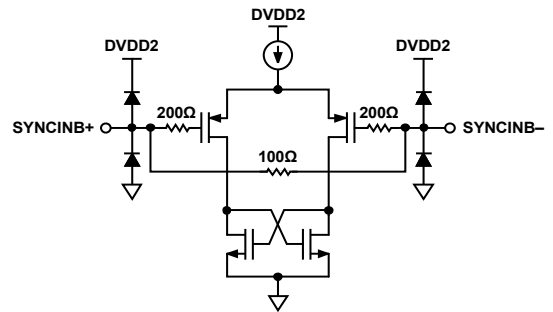
Figure 68. Equivalent SYNCIN<sub>±</sub> Input
