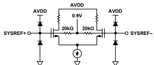
Figure 70. Equivalent SYSREF<sub>±</sub> Input Circuit
