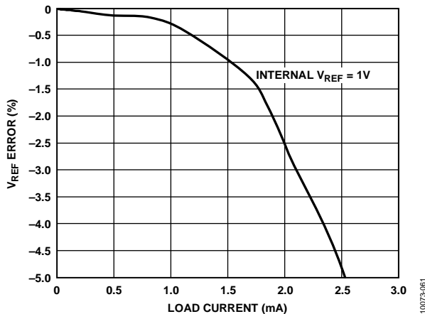
Figure 59. V_{REF} Error vs. Load Current
