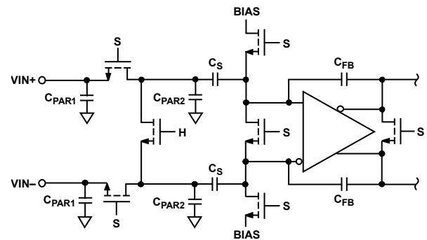
Figure 48. Switched-Capacitor Input
