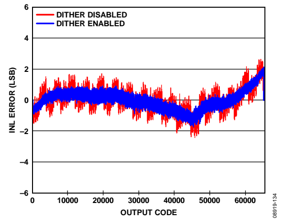
Figure 32. AD9650-65 INL with f_{IN} = 9.7 MHz
