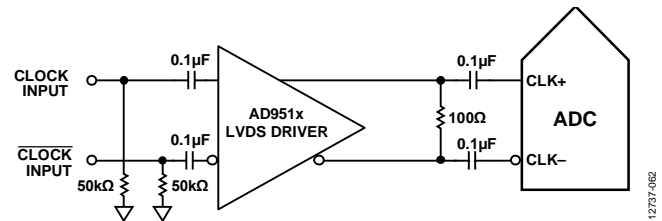
Figure 58. Differential LVDS Sample Clock (Up to 1 GHz)
