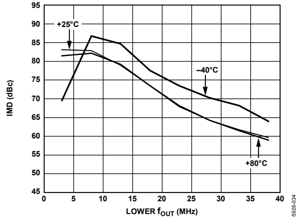
Figure 37. Dual-Tone IMD vs. Lower f_{OUT} and Temperature at 80 MSPS, I_{OUTFS} = 2 \text{ mA} and 0 dBFS
