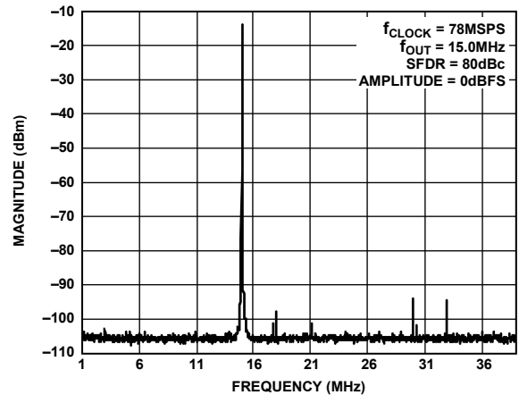
Figure 24. Single-Tone SFDR
