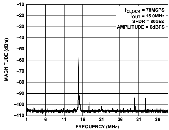
Figure 24. Single-Tone SFDR
