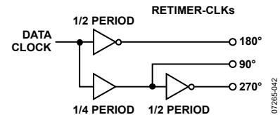
Figure 95. RETIMER-CLK Phases
