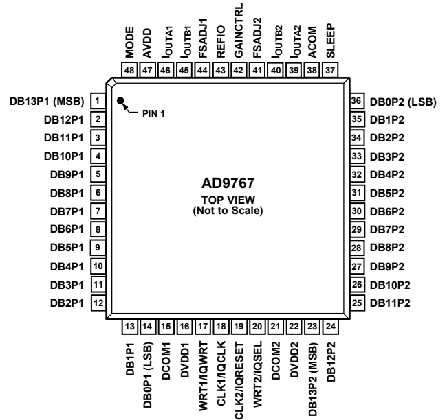
Figure 5. AD9767 Pin Configuration
