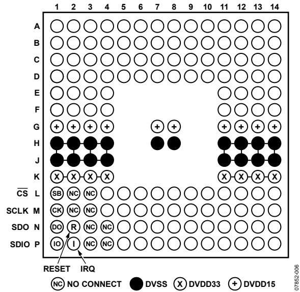
Figure 6. Digital Supply and SPI Pins (Top View)
