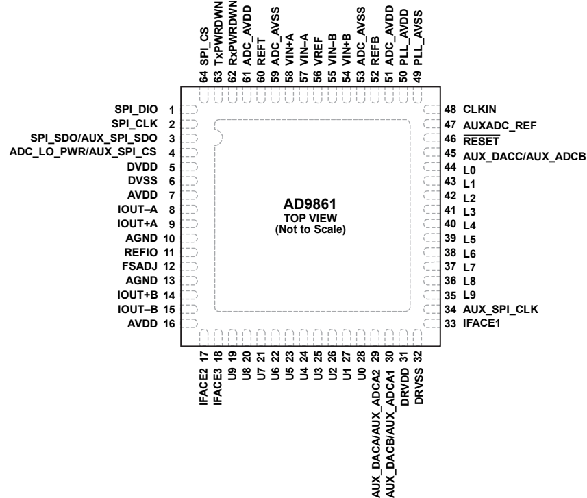
Figure 3. Pin Configuration
