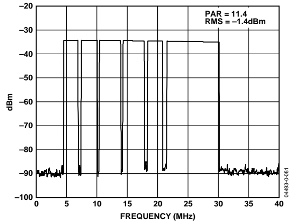
Figure 36. Spectral Plot of 111-Carrier OFDM Test Vector ( f_{DATA} = 80 MSPS, 2× Interpolation)
