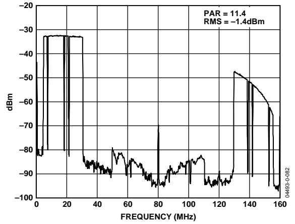
Figure 37. Wideband Spectral Plot of 111-Carrier OFDM Test Vector ( f_{DATA} = 80 MSPS, 2× Interpolation)
