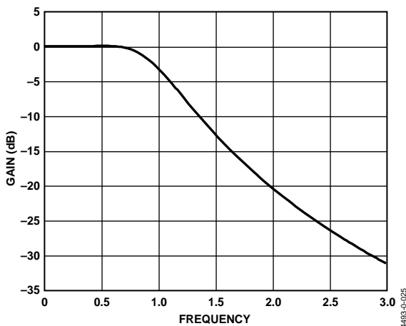
Figure 70. LPF's Normalized Wideband Gain Response
