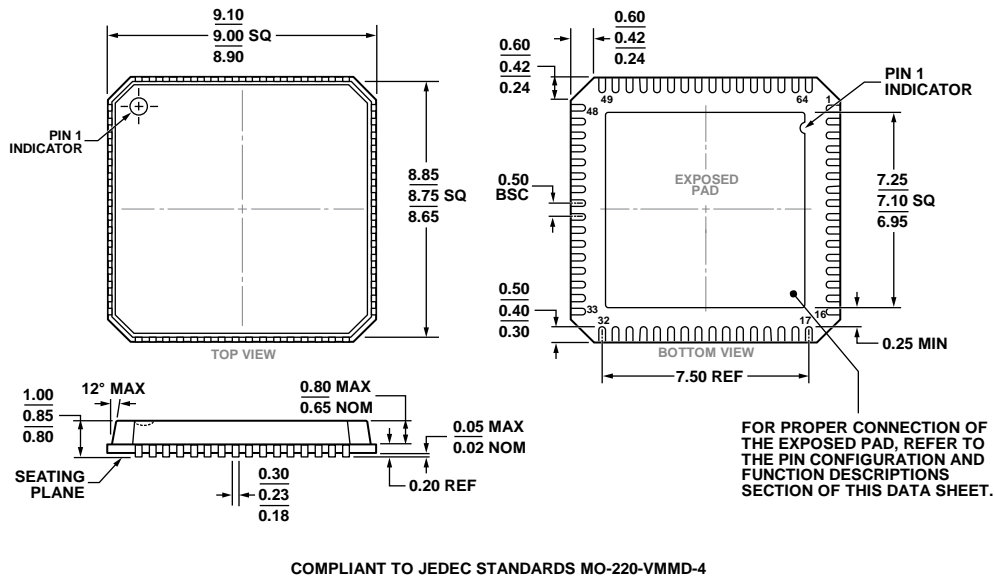
Figure 85. 64-Lead Lead Frame Chip Scale Package (LFCSP) 9 mm × 9 mm and 0.85 mm Package Height [CP-64-3] Dimensions shown in millimeters
