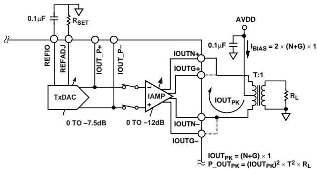
Figure 64. Current-Mode Operation
