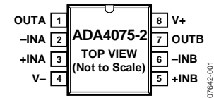
Figure 1. 8-Lead SOIC
