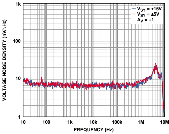
Figure 47. Voltage Noise Density vs. Frequency, V_{SY} = \pm 5V and V_{SY} = \pm 15V
