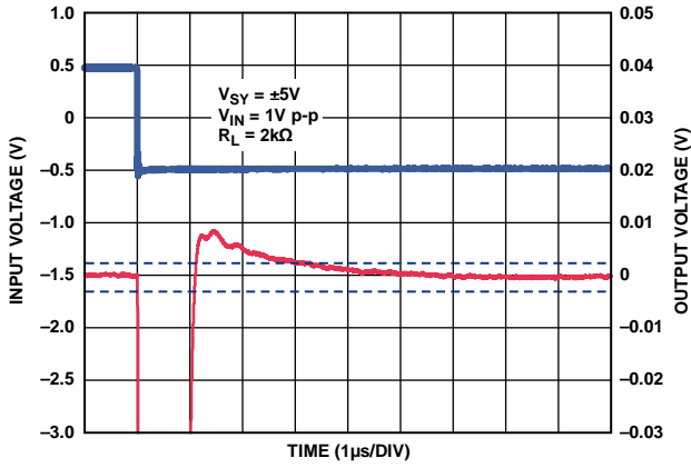
Figure 46. Negative 0.1% Settling Time, V_{SY} = \pm 5V
