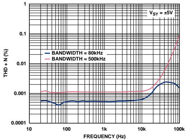
Figure 48. THD + N vs. Frequency, V_{SY} = \pm 5V
