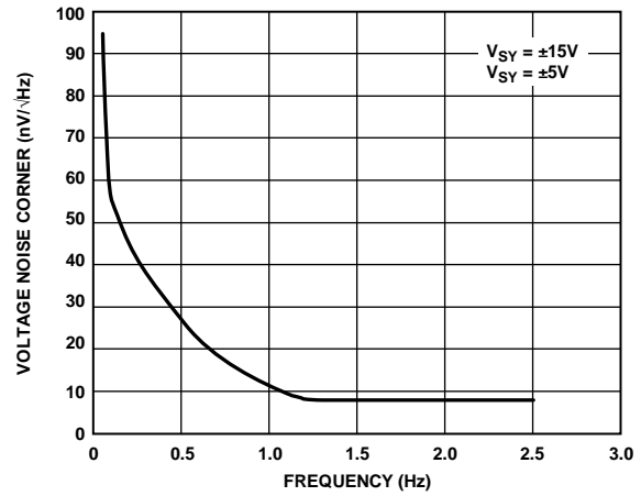
Figure 50. Voltage Noise Corner vs. Frequency, V_{SY} = \pm 15V and V_{SY} = \pm 5V
