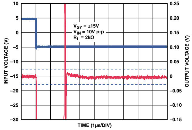
Figure 49. Negative 0.1% Settling Time, V_{SY} = \pm 15V
