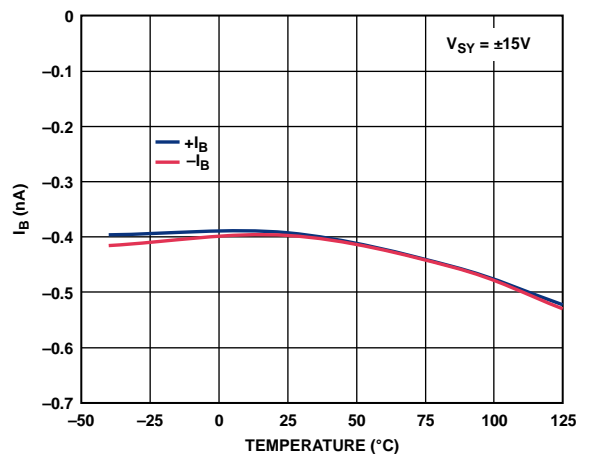
Figure 28. Input Bias Current ( I_b ) vs. Temperature, V_{SY} = \pm 15V
