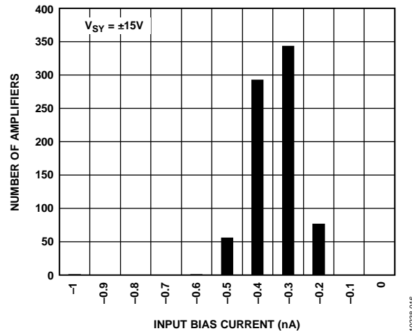
Figure 27. Input Bias Current Distribution, V_{SY} = \pm 15V
