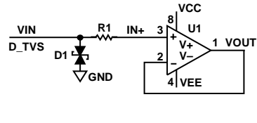
Figure 64. ESD Protection Circuit (R-TVS Network)
