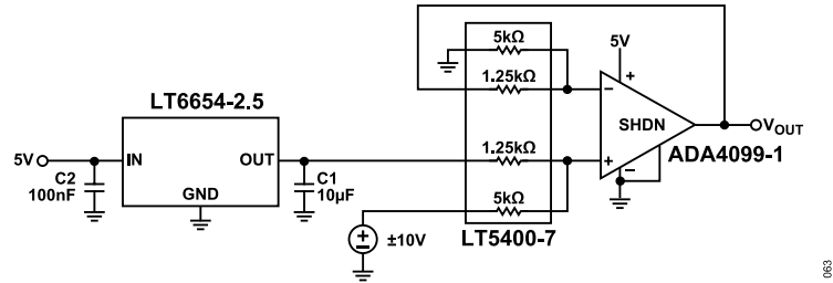
Figure 68. \pm 10 V to 0 V to +5 V Funnel Amplifier, High CMRR and \pm 80 V Input Protection via LT5400-7 Resistor Network (ADA4099-1 6-lead TSOT)
