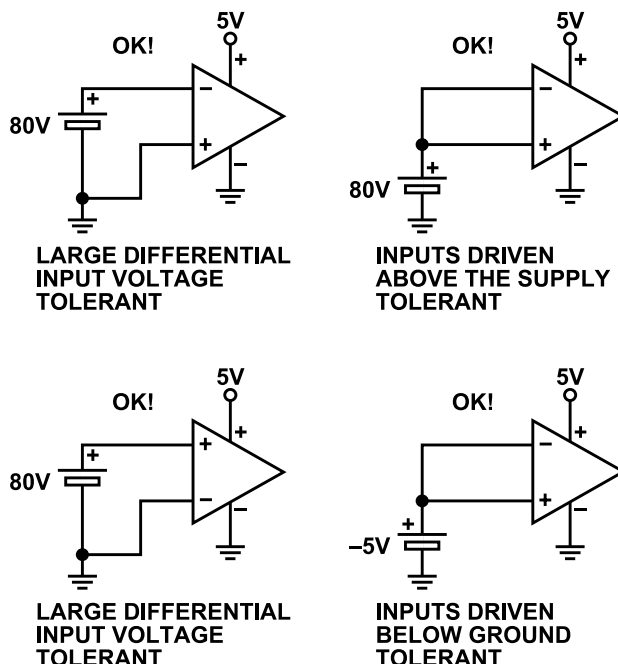
Figure 57. ADA4099-1 and ADA4099-2 Fault Tolerant Conditions
