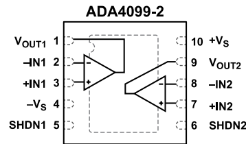
Figure 6. Pin Configuration for ADA4099-2 10-Lead LFCSP
