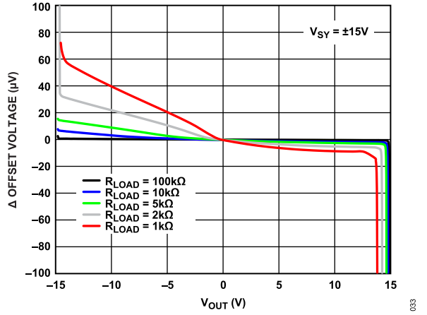
Figure 34. Δ Offset Voltage vs. Output Voltage ( V_{OUT} )
