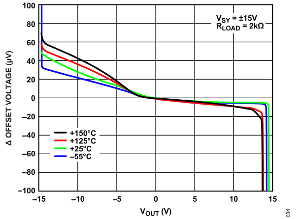
Figure 35. Δ Offset Voltage vs. V_{OUT} (2 kΩ Load)
