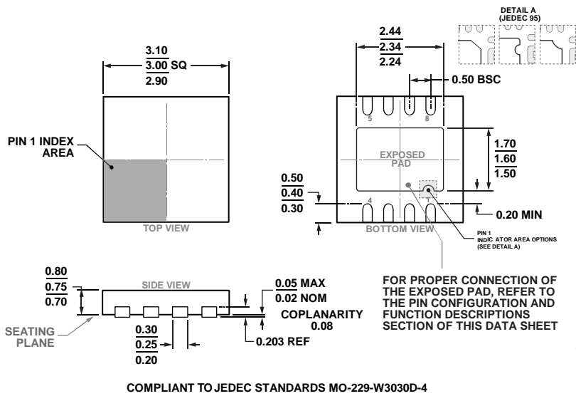
Figure 75. 8-Lead Lead Frame Chip Scale Package [LFCSP] 3 mm x 3 mm Body and 0.75 mm Package Height (CP-8-11) Dimensions shown in millimeters
