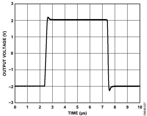
Figure 34. Large Signal Transient Response, V_{SY} = \pm 5\text{ V} , A_v = 1 , R_L = 2\text{ k}\Omega , C_L = 100\text{ pF}
