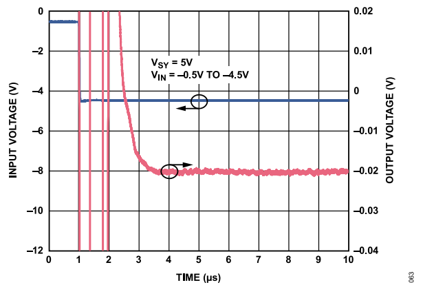
Figure 67. Negative Settling Time, A_V = -10 , V_{SY} = 5\text{ V}
