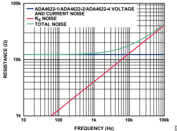
Figure 84. Total Noise vs. Source Resistance and Frequency
