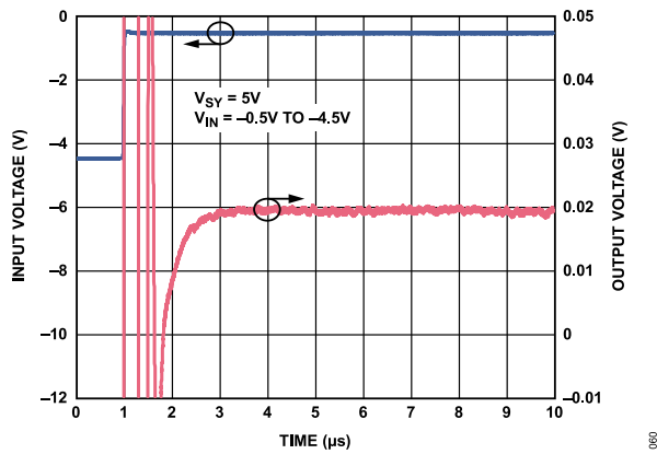
Figure 64. Positive Settling Time, A_V = -10 , V_{SY} = 5\text{ V}
