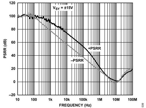
Figure 43. PSRR vs. Frequency, V_{SY} = \pm 15\text{ V}
