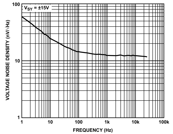
Figure 68. Voltage Noise Density, V_{SY} = \pm 15\text{ V}
