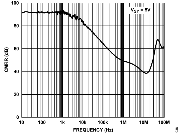
Figure 42. CMRR vs. Frequency, V_{SY} = 5\text{ V}
