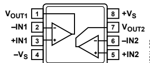
Figure 2. 8-Lead MSOP Pin Configuration (ADA4807-2)
