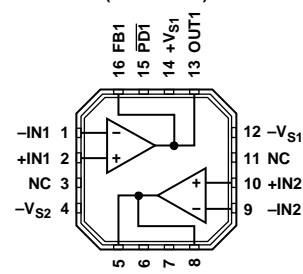
ADA4817-2 TOP VIEW (Not to Scale)
