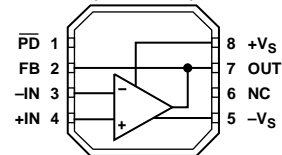
ADA4817-1 TOP VIEW (Not to Scale)
