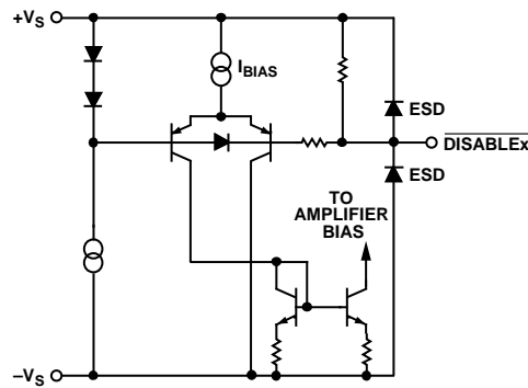
Figure 45. DISABLEx Circuit
