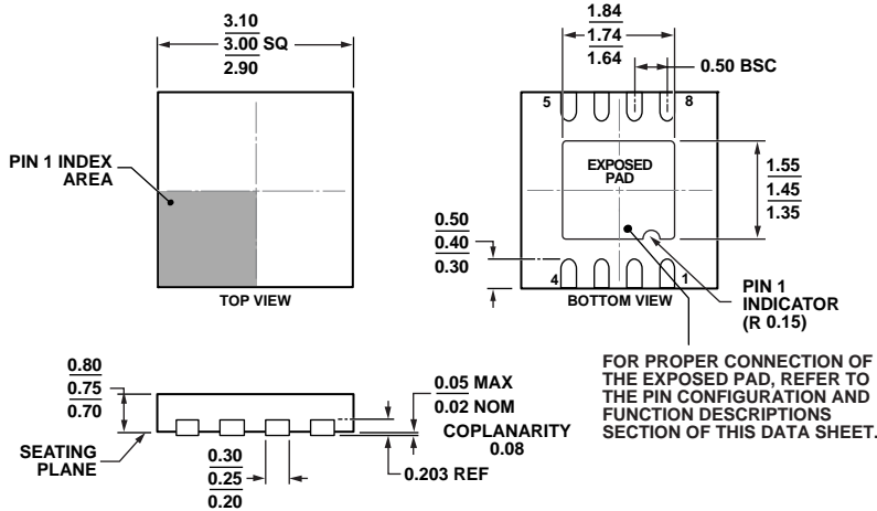
COMPLIANT TO JEDEC STANDARDS MO-229-WEED Figure 52. 8-Lead Lead Frame Chip Scale Package [LFCSPP] 3 mm x 3 mm Body and 0.75 mm Package Height (CP-8-13) Dimensions shown in millimeters
