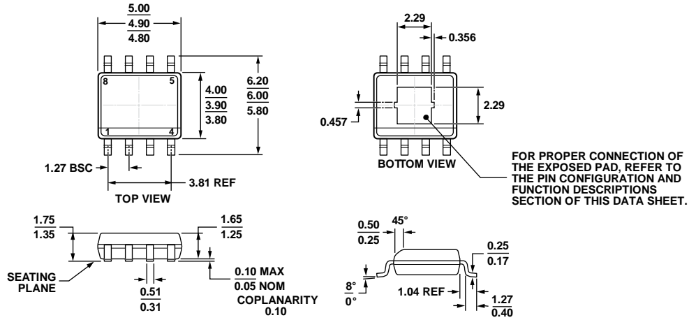
COMPLIANT TO JEDEC STANDARDS MS-012-AA Figure 51. 8-Lead Standard Small Outline Package with Exposed Pad [SOIC_N_EP] Narrow Body (RD-8-1) Dimensions shown in millimeters
