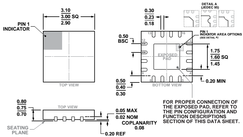
Figure 46. 16-Lead Lead Frame Chip Scale Package [LFCSP] 3 mm × 3 mm Body and 0.75 mm Package Height (CP-16-22) Dimensions shown in millimeters
