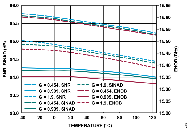
Figure 19. SNR, SINAD, and ENOB vs. Temperature, G = 1.9 , G = 0.909 , and G = 0.454 , f_{IN} = 1 \text{ kHz}
