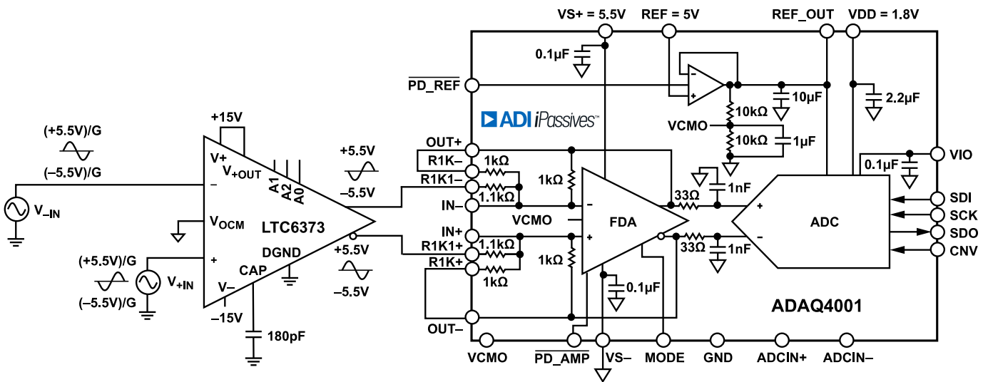
Figure 51. LTC6373 Driving ADAQ4001 (G = 0.454)
