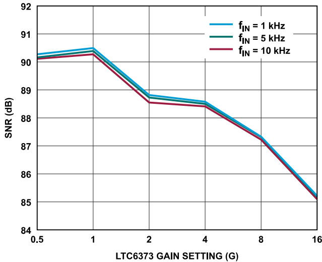
Figure 49. SNR vs. LTC6373 Gain Setting, LTC6373 Driving the ADAQ4001 (Gain = 0.454)
