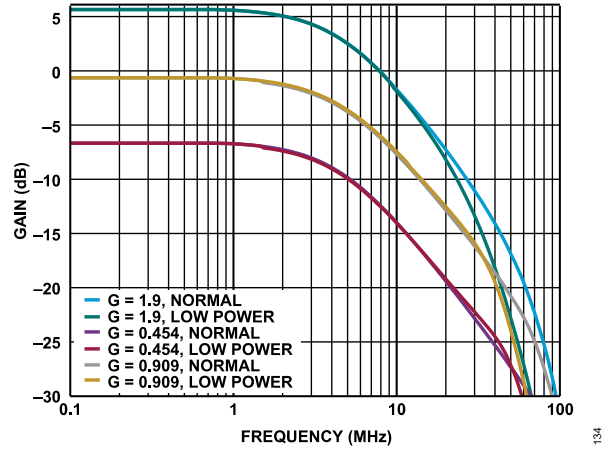
Figure 38. Small Signal Frequency Response and 0.1 dB Flatness for G = 1.9 , G = 0.454 , and G = 0.909 at Normal and Low Power Mode
