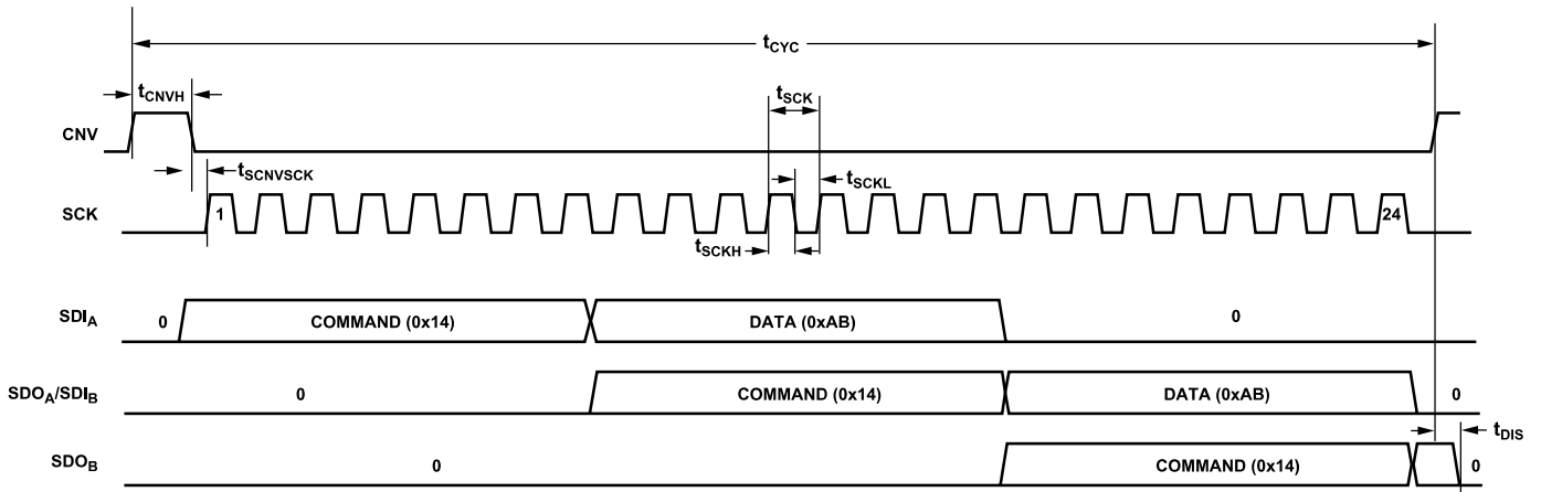
Figure 54. Register Write Timing Diagram, Daisy-Chain Mode
