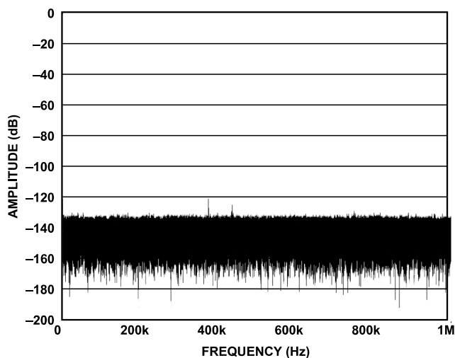
Figure 70. FFT with Shorted Inputs
