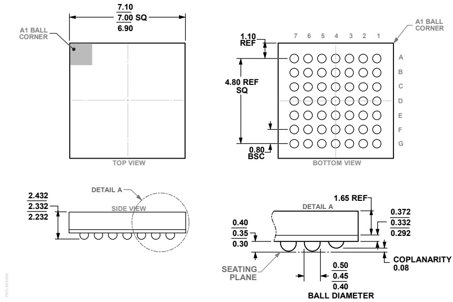
Figure 71. 49-Ball Chip Scale Package Ball Grid Array [CSP_BGA] (BC-49-5) Dimensions shown in millimeters
