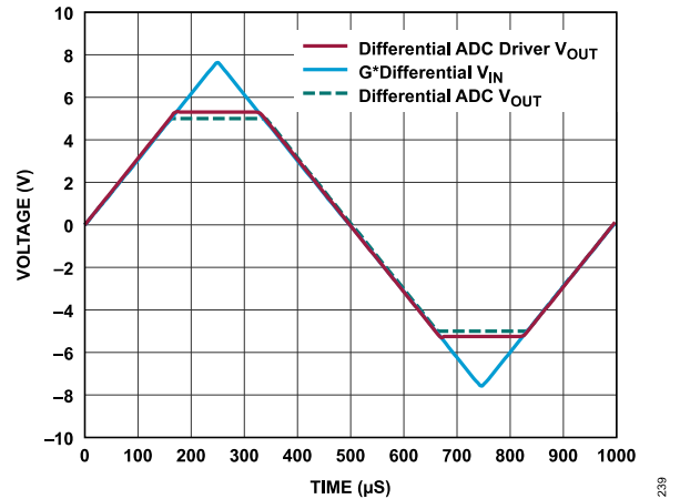
Figure 39. Output Drive Recovery, f_{IN} = 1 kHz
