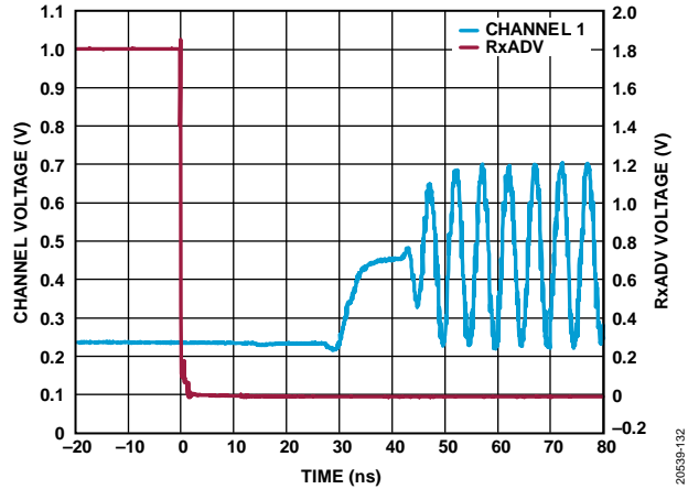
Figure 36. Receiver Sleep to Active Switching Time
