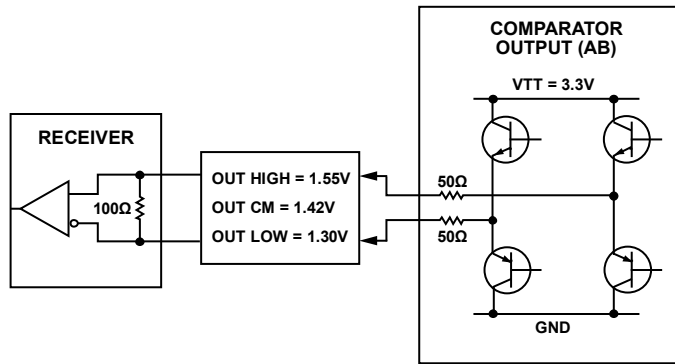
Figure 82. Comparator Output Scheme
