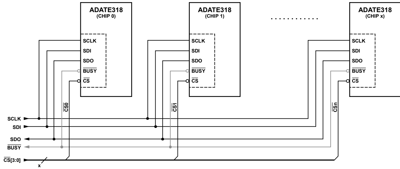
Figure 113. Multiple SPI with Shared SDO Line
