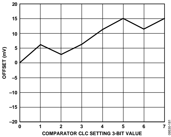
Figure 88. Normal Window Comparator Offset Error vs. CLC Setting
