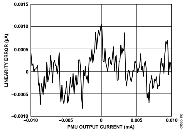
Figure 62. PPMU Range D Force Current Linearity Error
