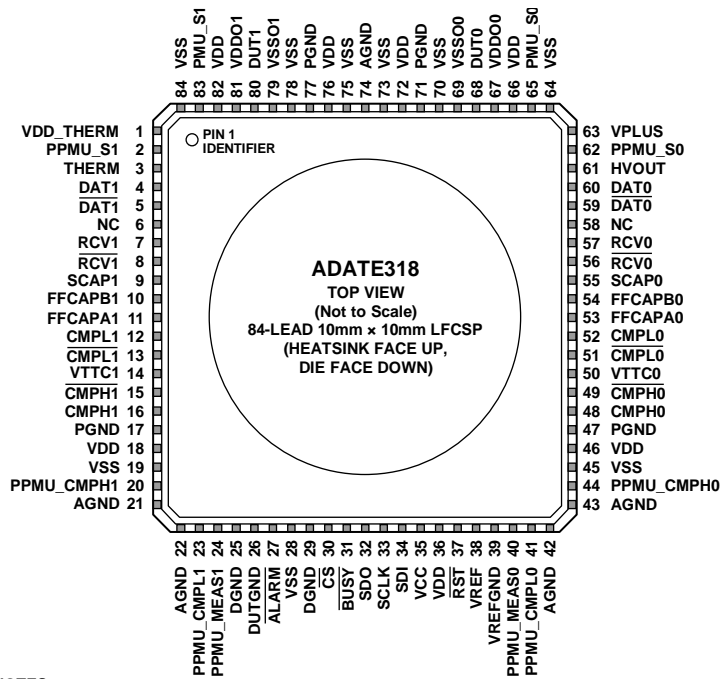
Figure 8. LFCSP Pin Configuration
