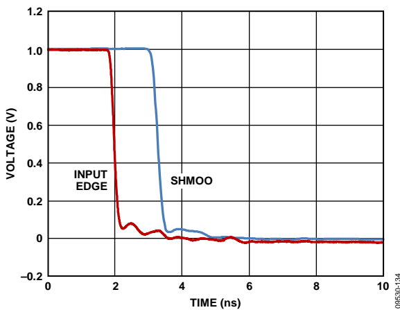
Figure 41. Normal Window Comparator Shmoo 1.0 V Swing; 50 Ω Termination, 200 ps (20% to 80%)
