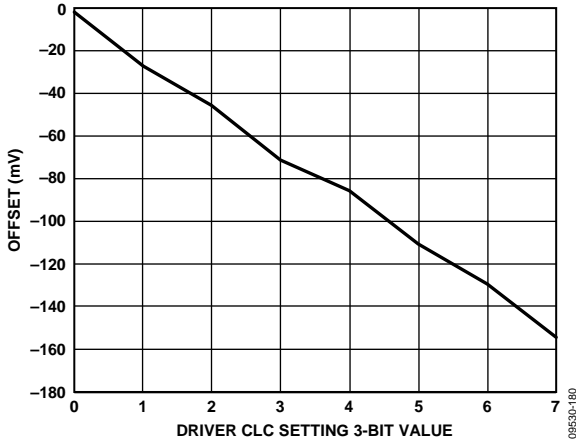
Figure 87. Driver Offset Error vs. Driver CLC Setting
