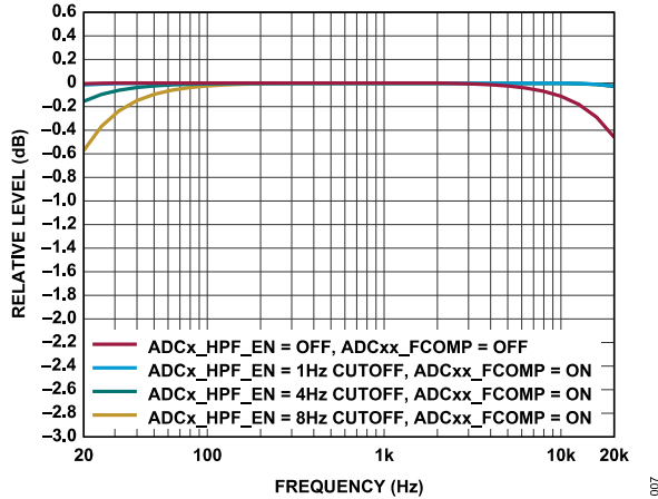
Figure 7. Frequency Response, f_s = 48 kHz, -20 dBV Input, Signal Path = AINx to SDATA0, No PGA, ADC0 and ADC1 Differential Mode, ADC2 Single-Ended Mode
