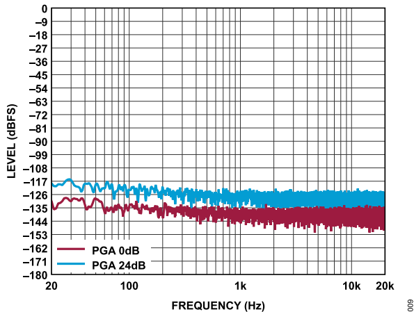
Figure 9. FFT, No Signal, f_s = 48 kHz, Signal Path = AINx to SDATA0, PGA = 0 dB and 24 dB (PGAx_GAIN), ADC0 and ADC1 Differential Mode
