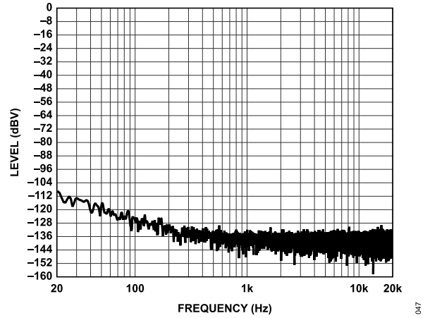
Figure 47. FFT, -1 dBV, f_s = 48 kHz to 768 kHz, Signal Path = AINx to DAC Headphone Mode (16 Ω) or Line Output Mode (10 kΩ), ADC2 Single-Ended Mode
