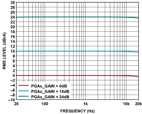
Figure 8. Frequency Response, f_s = 48 kHz, Signal Path = AINx to SDATA0, Output Relative to PGA Gain Settings (0 dB, 10 dB, 24 dB)
