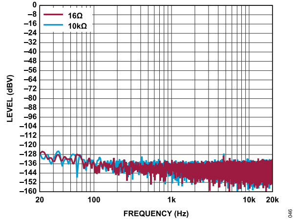
Figure 46. FFT, -1 dBV, f_s = 48 kHz to 768 kHz, Signal Path = AINx to DAC Headphone Mode (16 Ω) or Line Output Mode (10 kΩ), ADC0 and ADC1 Differential Mode
