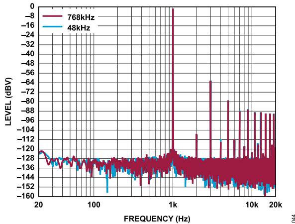
Figure 44. FFT, -1 dBV, Headphone Mode, Load = 16 Ω, f_s = 48 kHz to 768 kHz, Signal Path = AINx to DAC, ADC0 and ADC1 Differential Mode
