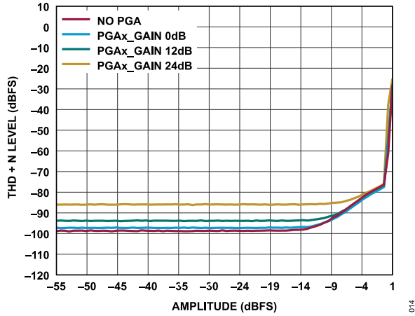
Figure 14. THD + N Level vs. Amplitude, f_s = 48 kHz, Signal Path = AINx to SDATA0, No PGA and PGA Gain Settings (0 dB, 12 dB, 24 dB), ADC2 Single-Ended Mode
