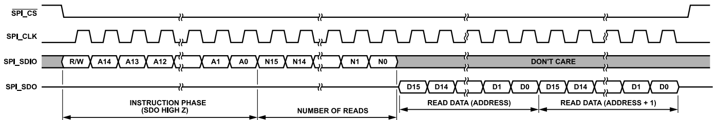
Figure 38. Basic 4-Wire Read Operation
