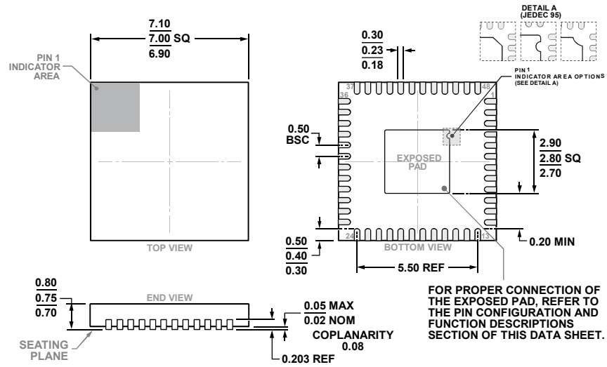
Figure 33. 48-Lead Lead Frame Chip Scale Package [LFCSP] 7 mm x 7 mm Body and 0.75 mm Package Height CP-48-21
