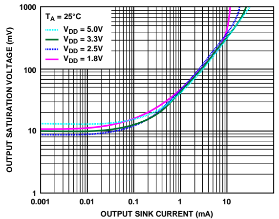
Figure 19. Output Saturation Voltage vs. Output Sink Current
