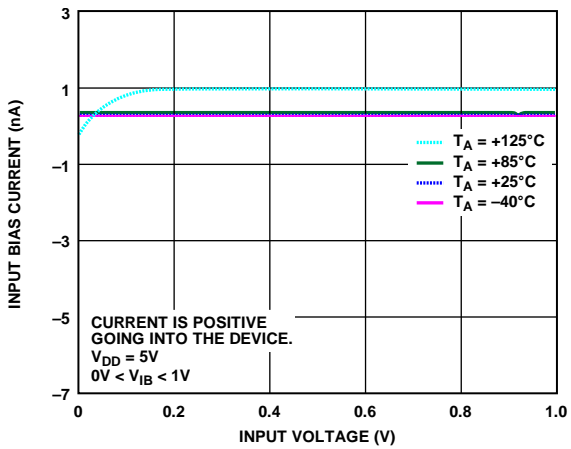
Figure 18. Low Level Input Bias Current
