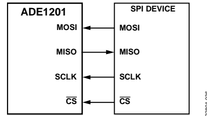
Figure 35. Connecting the SPI to an SPI Device
