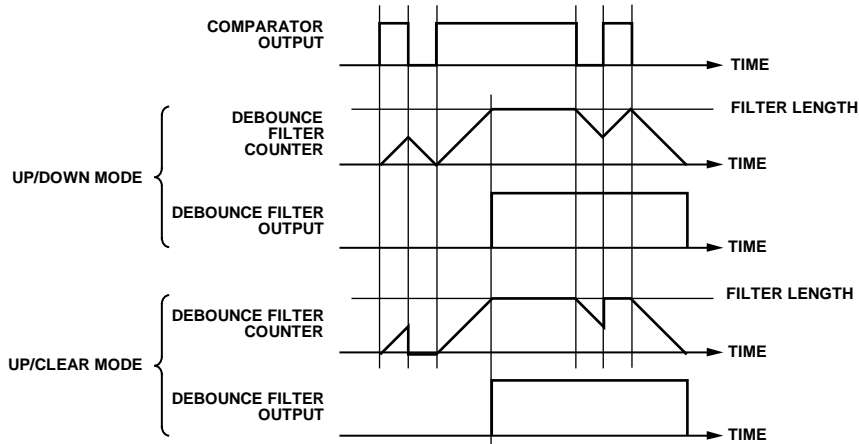
Figure 32. Debounce Filter Function Example
