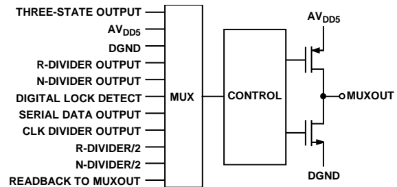
Figure 19. MUXOUT Schematic
