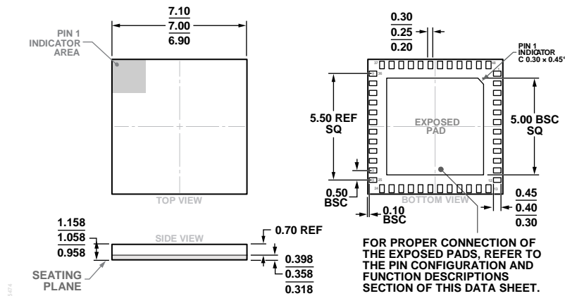
Figure 38. 48-Terminal Land Grid Array [LGA] (CC-48-4)
