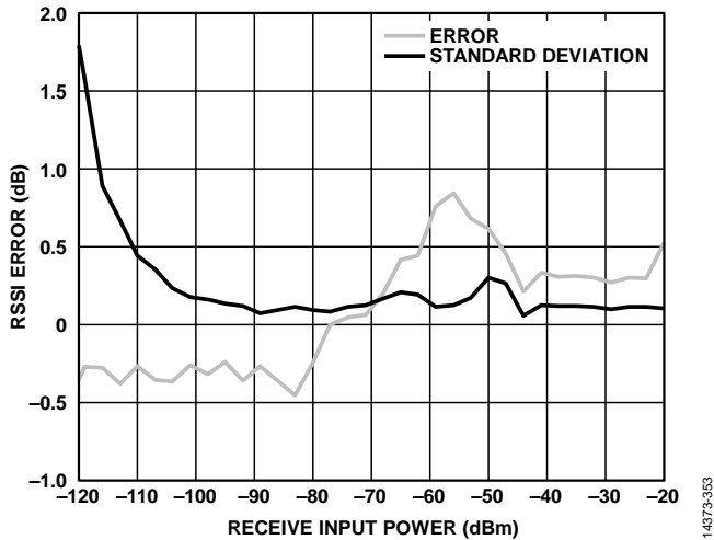
Figure 53. Packet RSSI Error vs. Rx Input Power with One-Point Calibration at -77 dBm; Configuration 868 MHz/4.8 kbps; V_{DD} = 3.0\text{ V} ; T_A = 25^\circ\text{C} (Error is Based on the Mean RSSI of 100 Packets)
