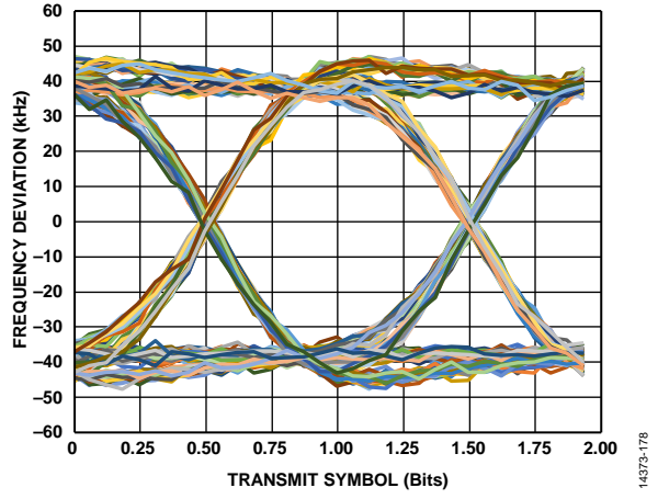
Figure 77. Transmit Eye Diagram, PA2 Output Power = 17 dBm, Configuration 915 MHz/150 kbps, V_{DD} = 3.0\text{ V} , T_A = 25^\circ\text{C}
