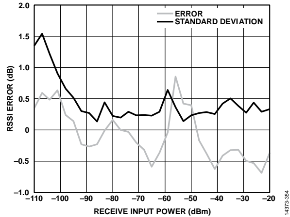
Figure 54. Packet RSSI Error vs. Rx Input Power with One-Point Calibration at -70 dBm; Configuration 868 MHz/100 kbps; V_{DD} = 3.0\text{ V} ; T_A = 25^\circ\text{C} (Error is Based on the Mean RSSI of 100 Packets)
