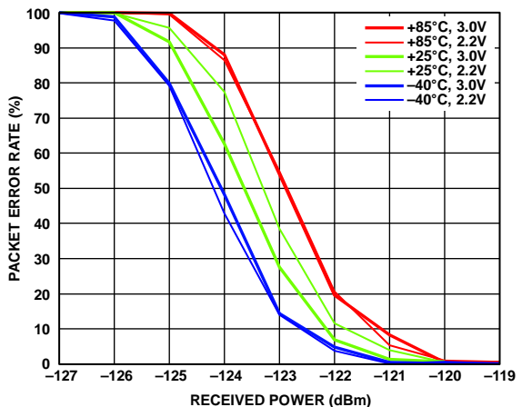
Figure 9. Packet Error Rate vs. RF Input Power, Temperature and VDD Configuration 169.43125 MHz/2.4 kbps
