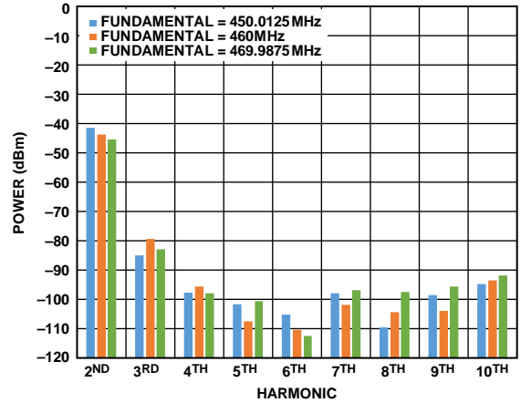
Figure 43. Conductive Harmonic Emission Level, PA2 Output Power = 17 dBm, RF Frequency = 460 MHz, V DD = 3.0 V, T A = 25°C
