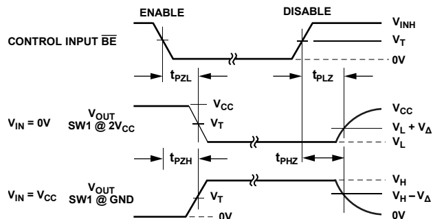
Figure 27. Enable and Disable Times
