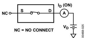
Figure 20. I_b (On)
