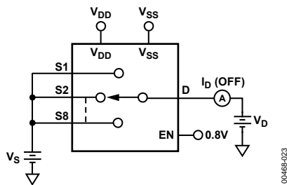
Figure 19. I_b (Off)
